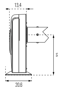
Electric support with colored disk
