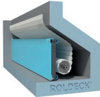
Recessed in cave with hinged front panel and nose wheel guides
