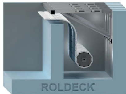
Below ground in pit cantilever brackets (letter box)
